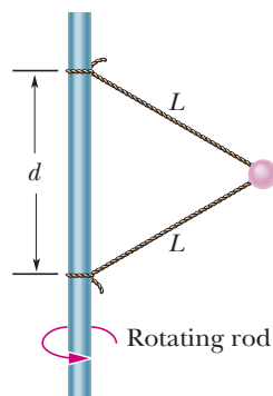
Figure 6-45 Problem 59.
