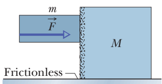
Figure 6-38 Problem 35.
