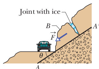
Figure 6-22 Problem 14.
