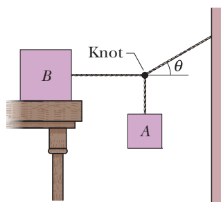
Figure 6-31 Problem 25.
