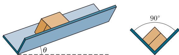
Figure 6-51 Problem 67.
