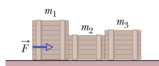
Figure 6-32 Problem 26.
