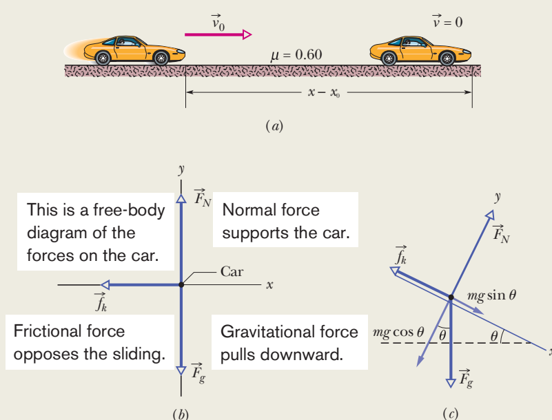
Figure 6-4 (a) A car sliding to the right and finally stopping after a displacement of 290 m. A free-body diagram for the car on (b) a horizontal road and (c) a hill.
