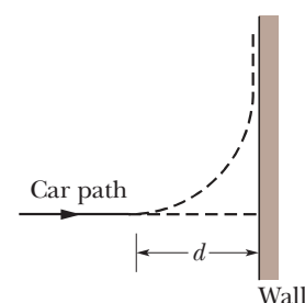
Figure 6-44 Problem 58.
